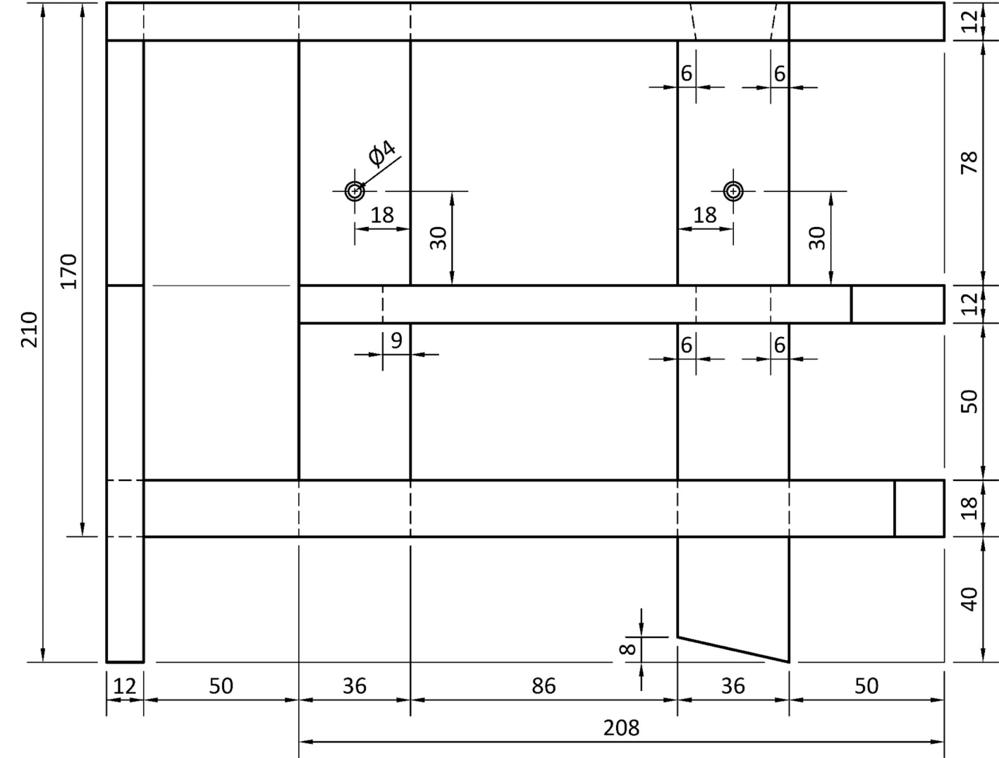
Elevation/Ingearchló
